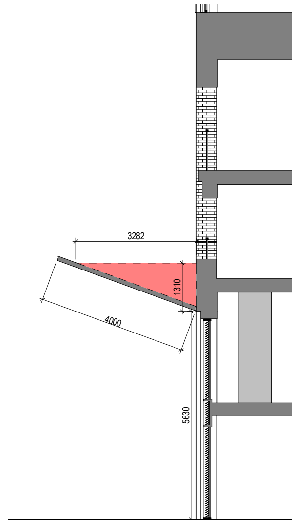
Proposed Section_AA
