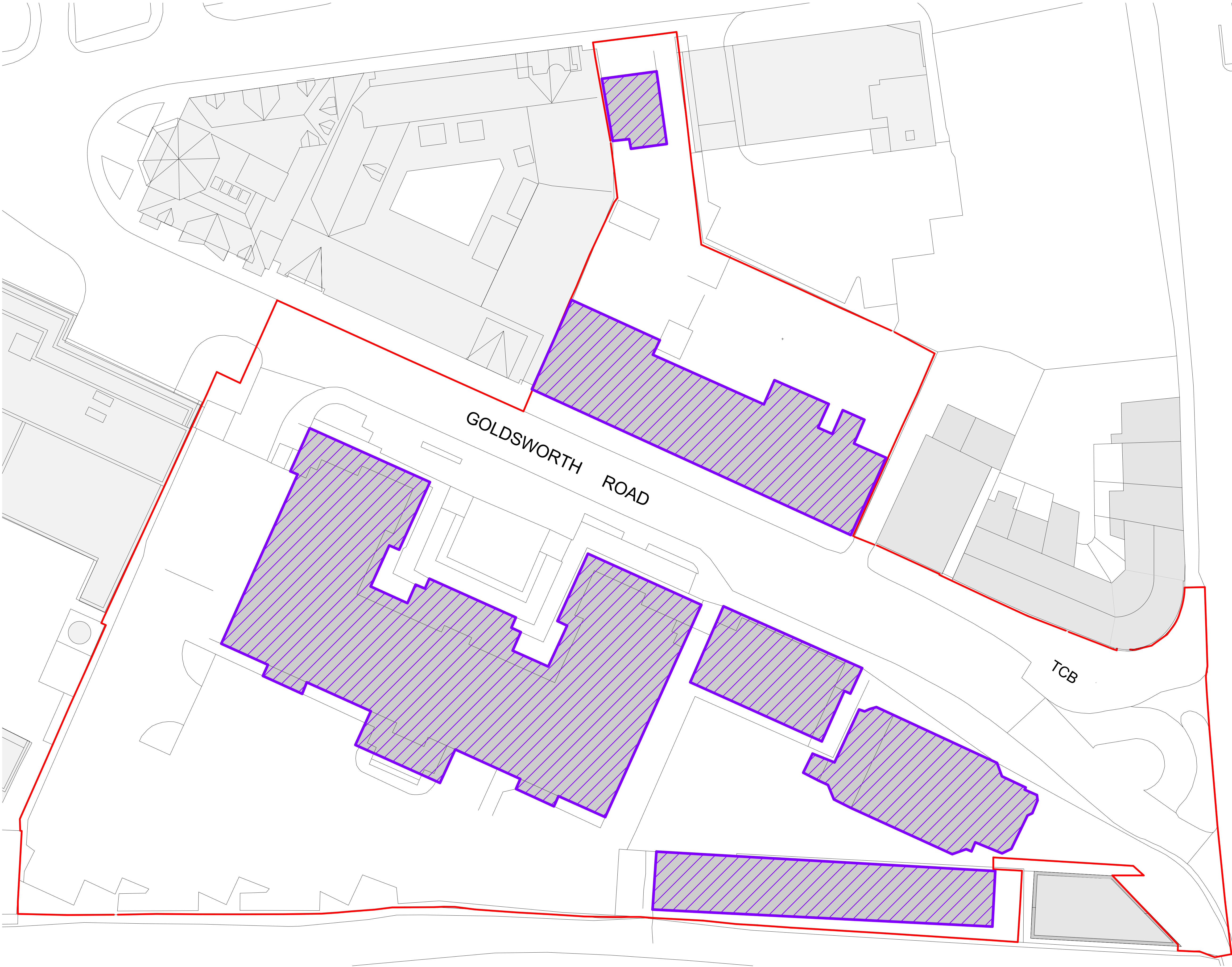
Proposed Phasing Plan - Phase 0 1 : 250
