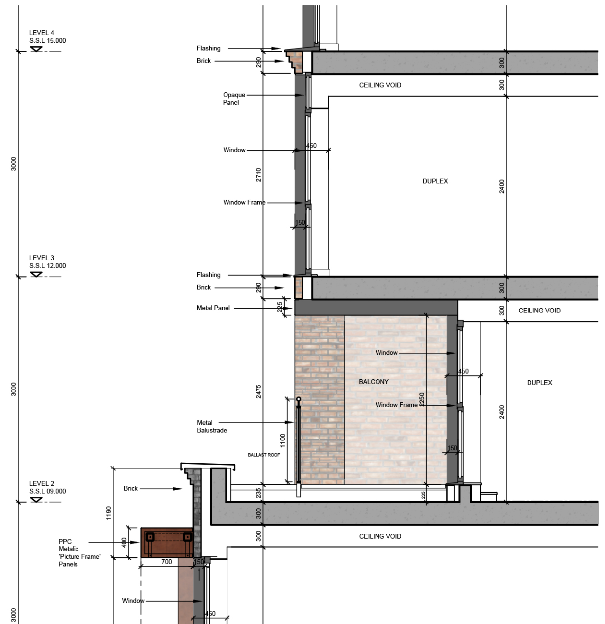
Typical Section A-A
