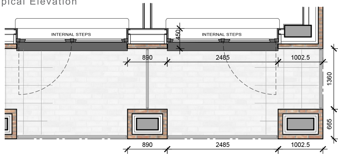
Typical Elevation
