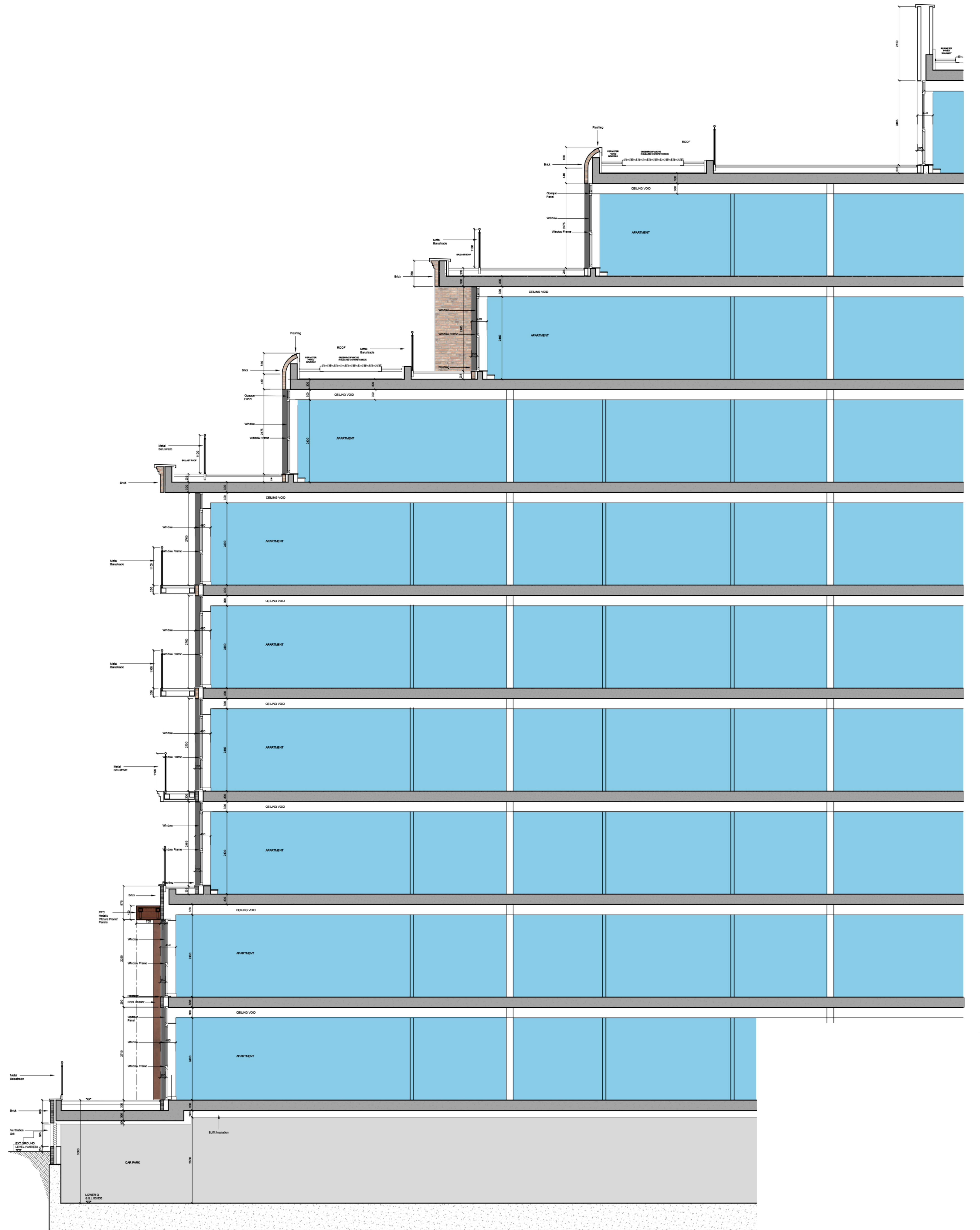
Typical Section A-A
