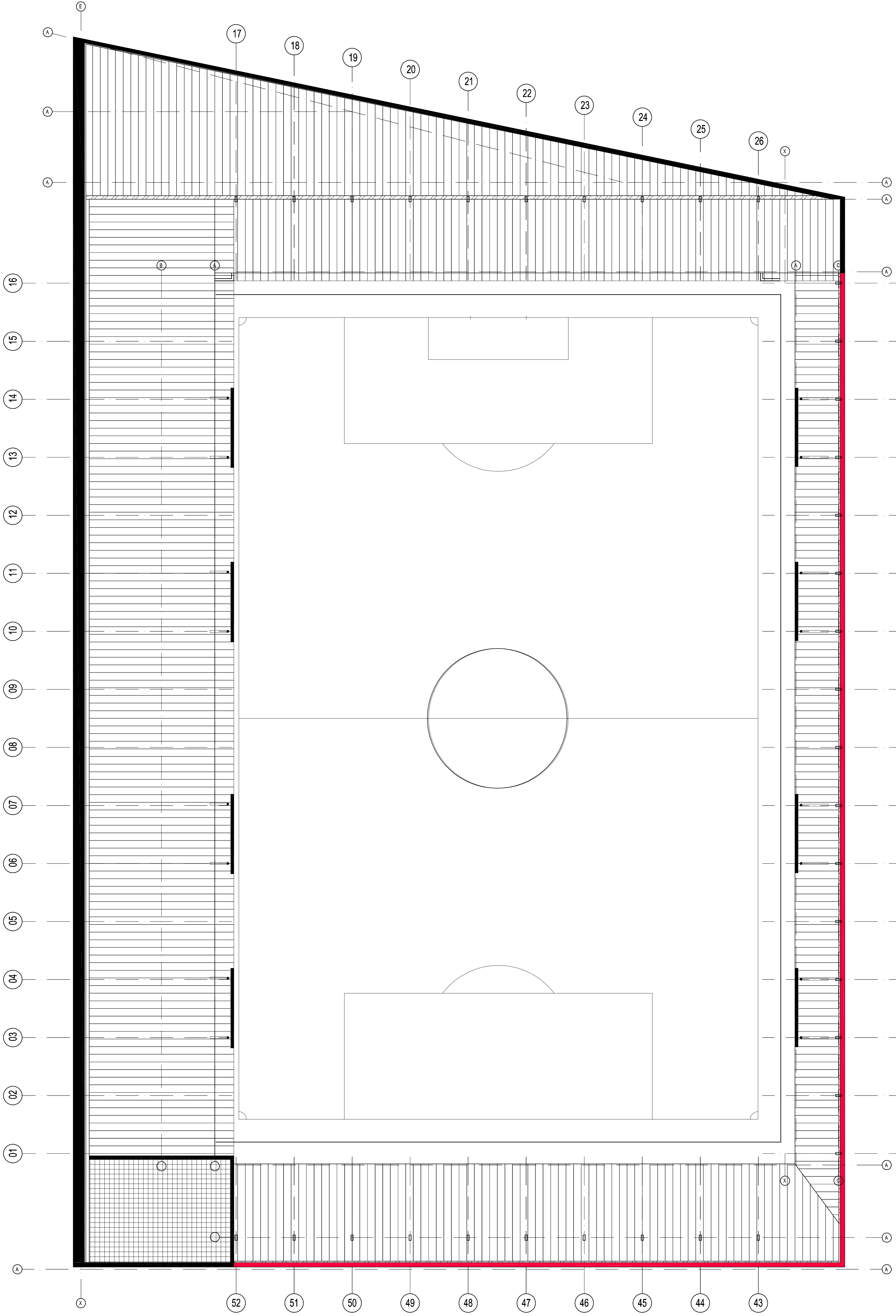
ROOF PLAN: WEST STAND
